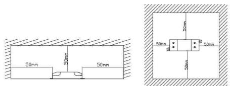
Mounting location dimension
